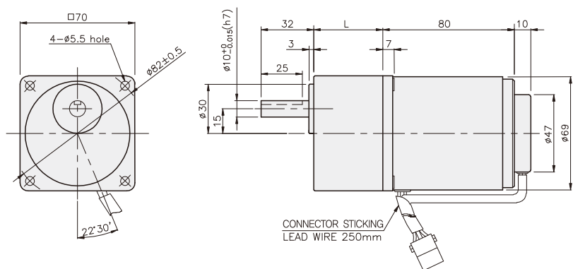
K7IG15N□-SU + K7G□B(C)
