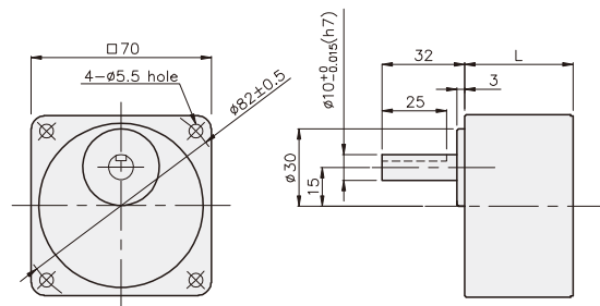
GEARHEAD K7G□B(C)
