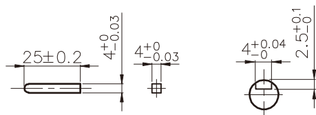
K7IG15N□-SU + K7G□B(C)
